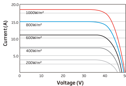
I-V CURVES OF PV MODULE (730W)
