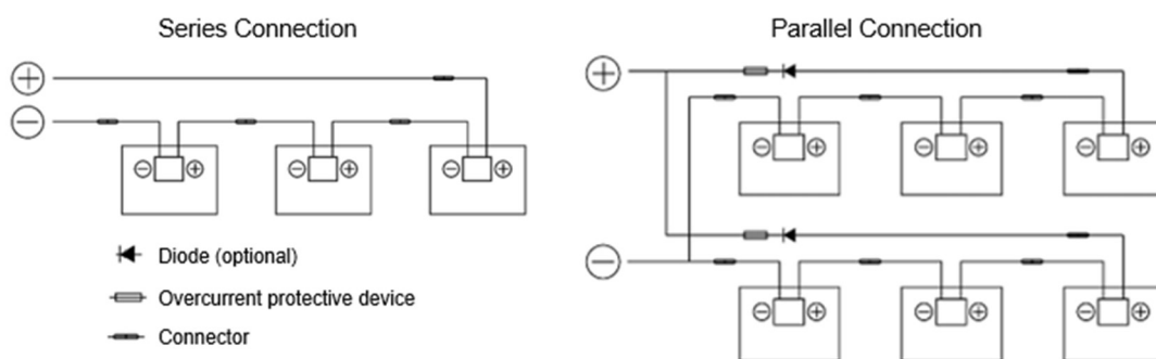
Figure 6. Series and parallel connection circuit diagram.
