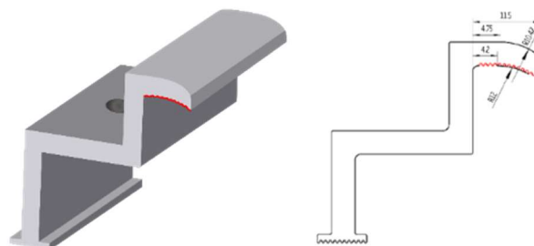
Figure 3. A surface matching clamp
