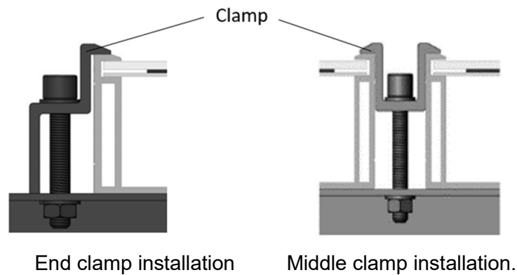
Figure 2. PV module installed with clamp fitting method
