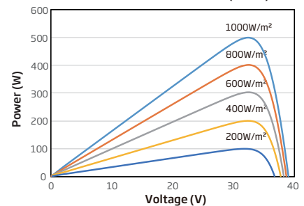
P-V CURVES OF PV MODULE (500W)
