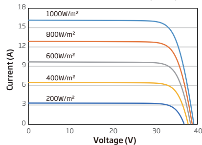
I-V CURVES OF PV MODULE (500W)
