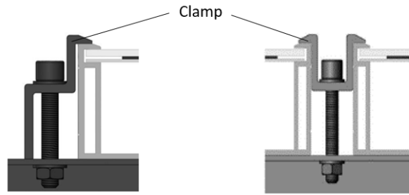
End clamp installation Middle clamp installation.
