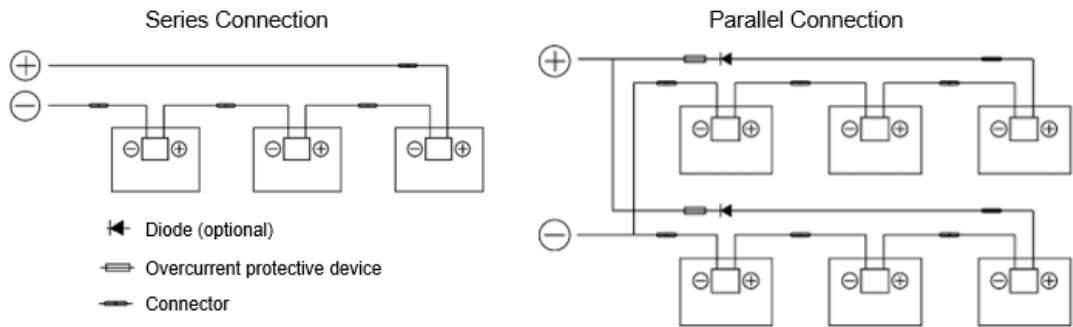
Figure 6. Series and parallel connection circuit diagram.
