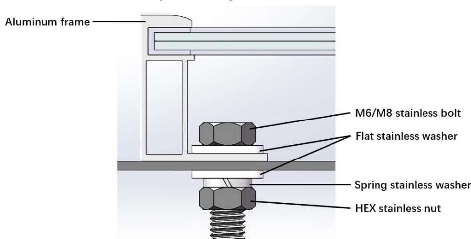
Figure 1. PV module installed with bolt fitting method.
