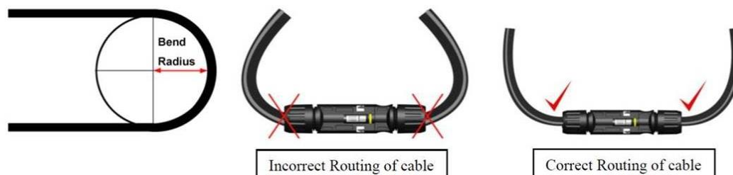
Figure 5. The correct routing and minimum bending radius of cables.
