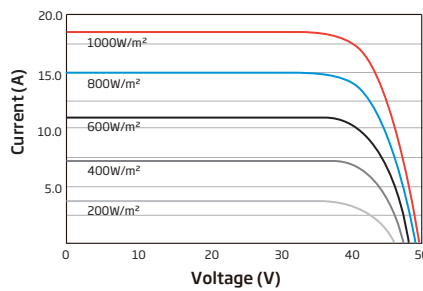
I-V CURVES OF PV MODULE (725W)
